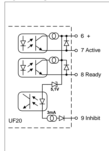
Fig. 10-2 Signals schematic
