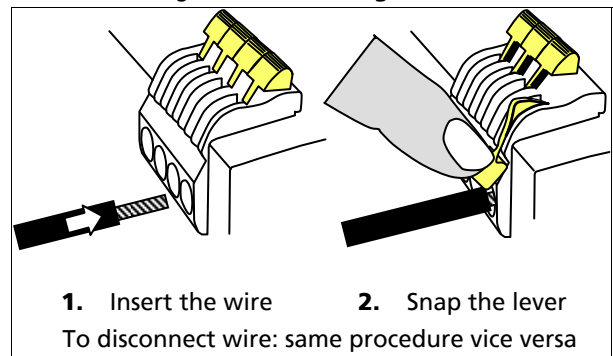
Fig. 12-1 Connecting a wire
