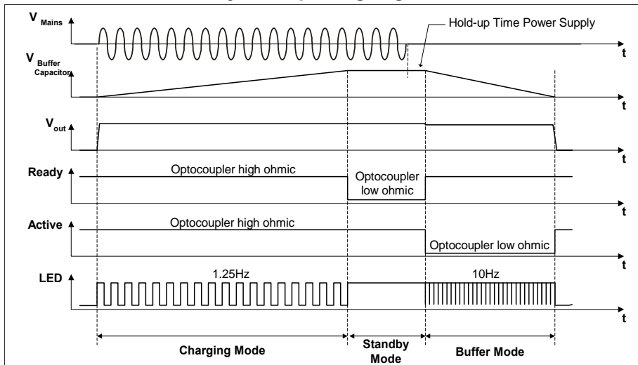
Fig. 10-1 Operating diagram
