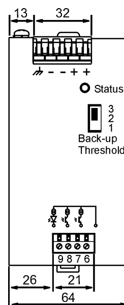
Fig. 20-2 Front view
