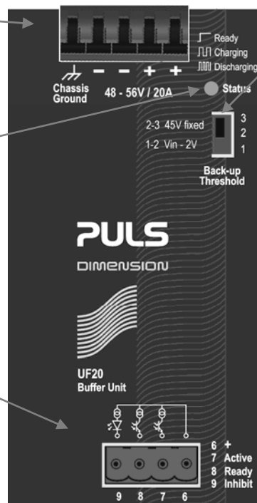
Fig. 9-1 Front side
