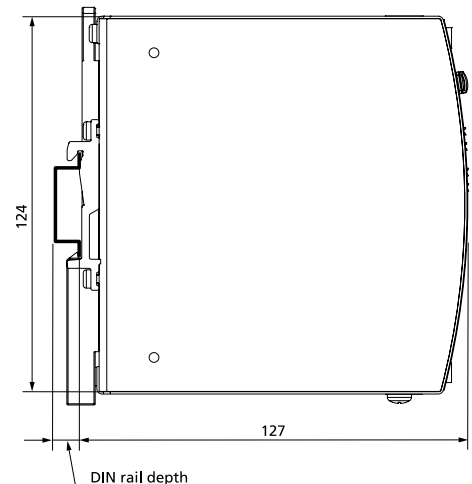
Fig. 23-5: Side view
