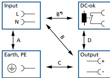
Fig. 20-1: Dielectric strength
