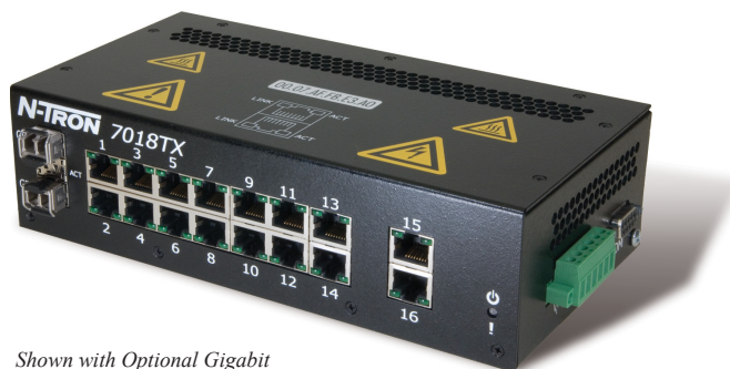
Shown with Optional Gigabit SFP Transceivers installed
