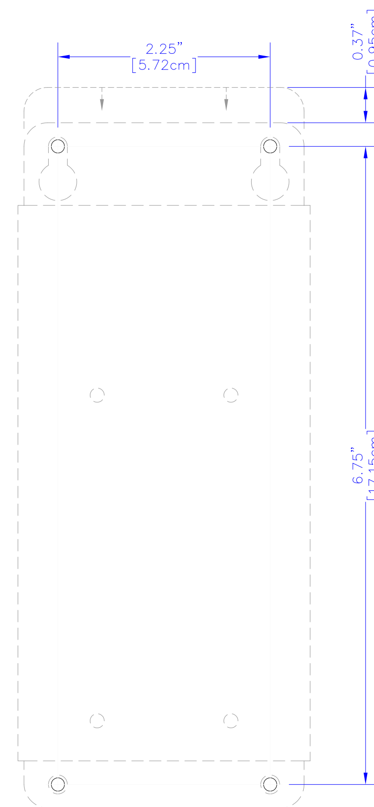
RECOMMENDED MOUNTING HOLE TEMPLATE
