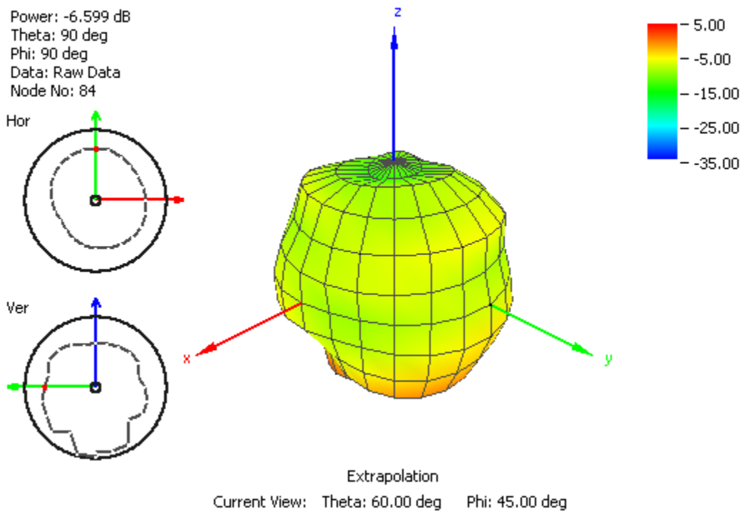
Figure21. Radiation Pattern at 1710 MHz of G30 Antenna in Free Space
