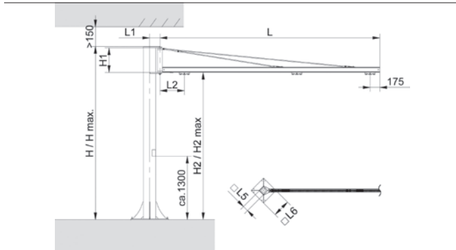
Column mounted jib crane SK
