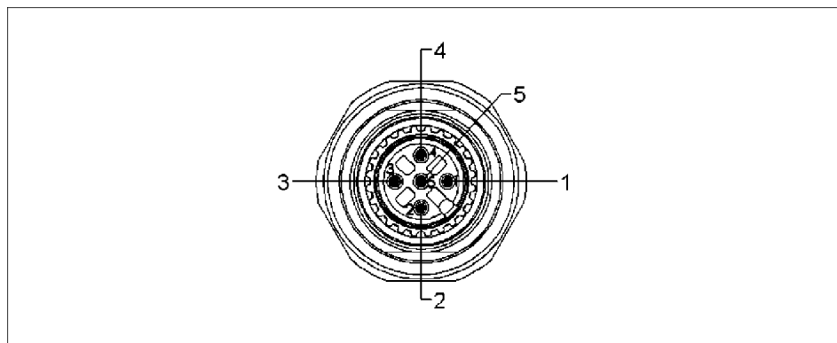
M12 5-Pin Female Euchner Safety Switch Connector
