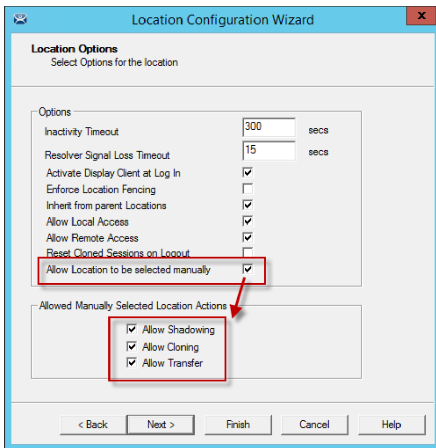
Location Options Page
