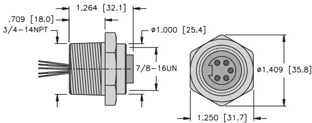
P-RKF .. 14.75/NPT
