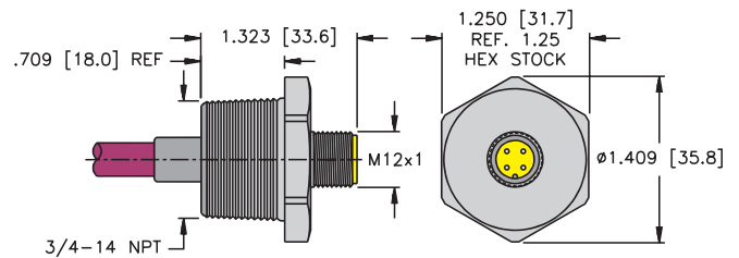
P-FS .. 14.75/NPT
