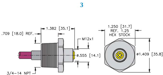
P-FK .. 14.5/NPT
