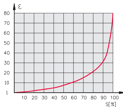
RELATION OF OPERATING DISTANCE TO DIELECTRIC CONSTANT
