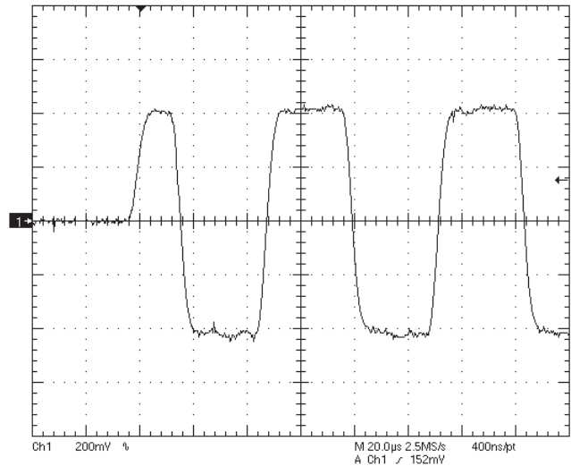
FOUNDATION fieldbus signal with both terminators correctly installed.
