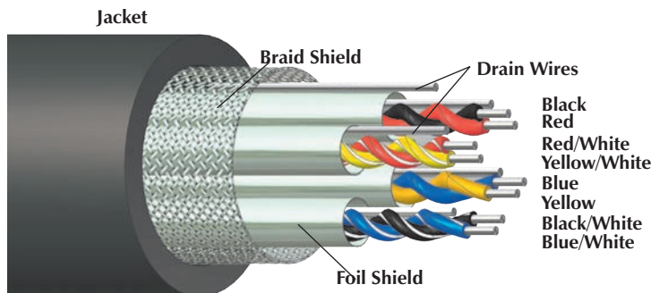
Example of Type B Cable
