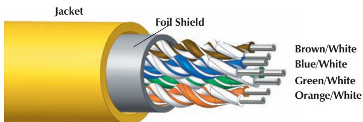
Example of Type C Cable
