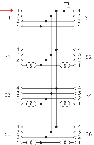
Circuit diagram of a TURCK multiport junction box with current limited drops.
