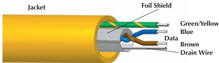
Example of Type A Cable
