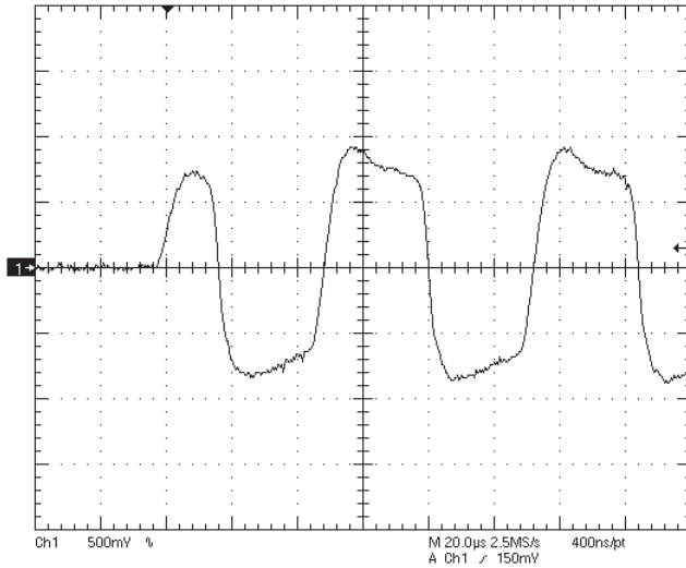
FOUNDATION fieldbus signal with only one terminator in place.
