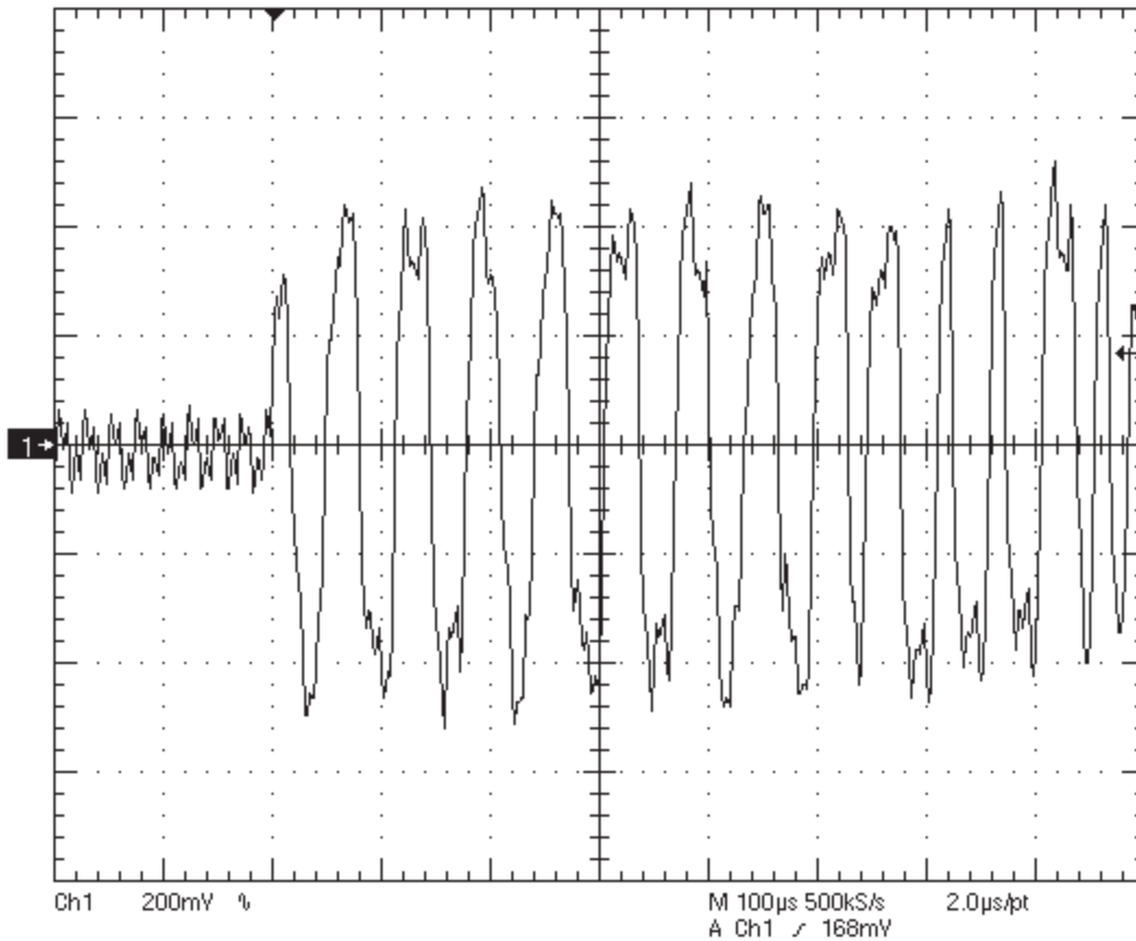
Real world FOUNDATION fieldbus signal with noise present.
