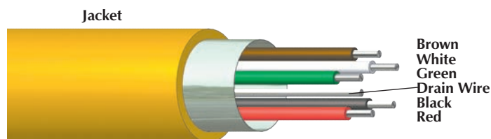
Example of Type D Cable
