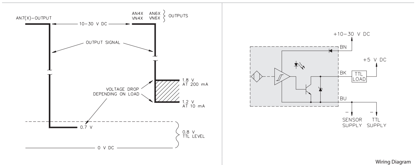
Wiring Diagram
