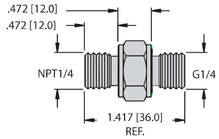
PCV-N1/4A4 | A9867
