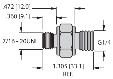
PCV-S7/16A4 | A9136
