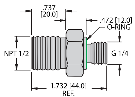
PCV-N1/2A4 | M6835013
