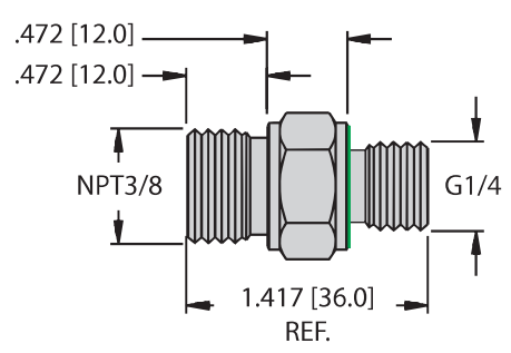
PCV-N3/8A4 | M6835020
