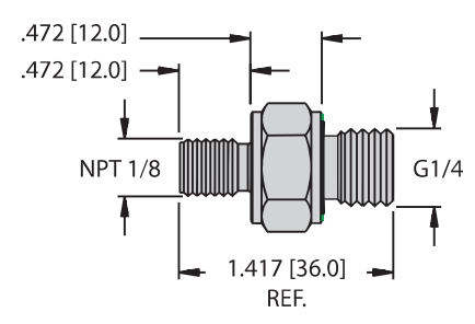
PCV-N1/8A4 | M6835021
