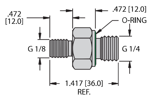
PCV-G1/8A4 | M6835014
