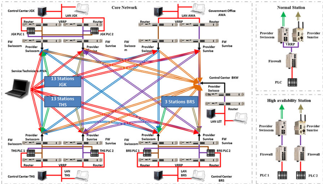
The main control network incorporates the AWA control centre in the capital, Berne, and further control centres at the water locks, 29 substations 8 SCADA clients, and a SCADA server in hydropower plant. Image:AWA
