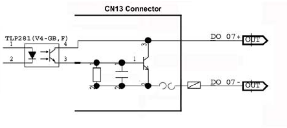
Digital Output Circuit
