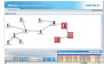
Event Playback
