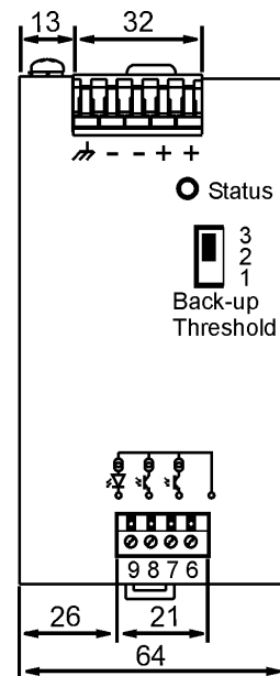
Fig. 20-2 Front view
