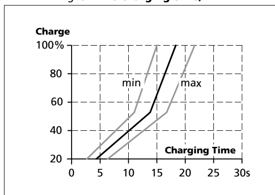
Fig. 6-1 Re-charging time, 24V
